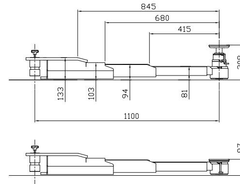
Short arm
